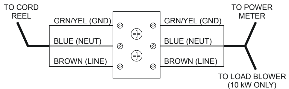
Figure 8 Cal Cart Wiring Schematic
